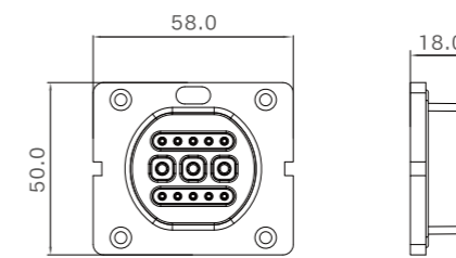
Male Size
