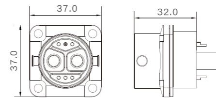
Female Size
