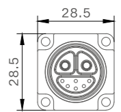
Female Size
