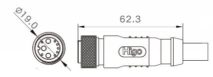
Female Size
