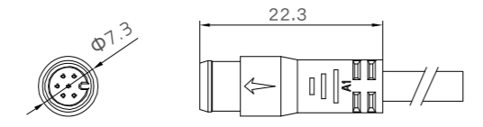
Male Size
