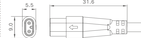
Male Size
