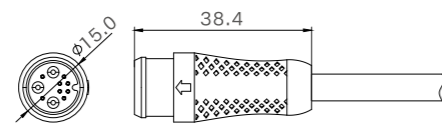
Male Size
