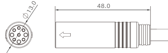
Female Size
