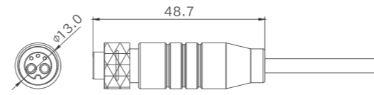
Female Size
