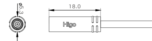
Male Size
