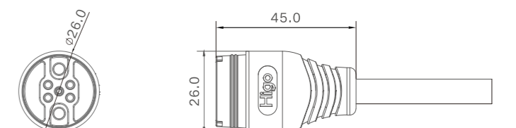
Female Size
