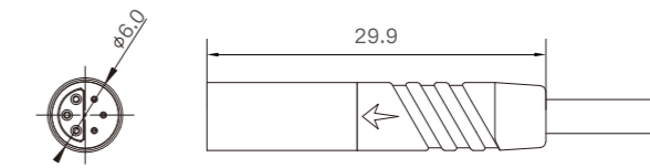
Male Size
