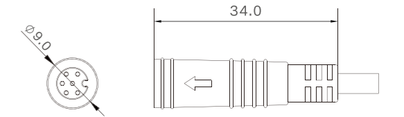
Female Size
