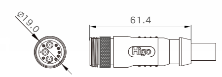
Male Size
