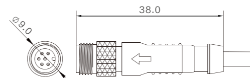
Male Size
