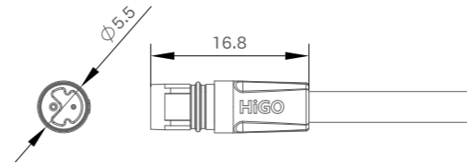
Female Size
