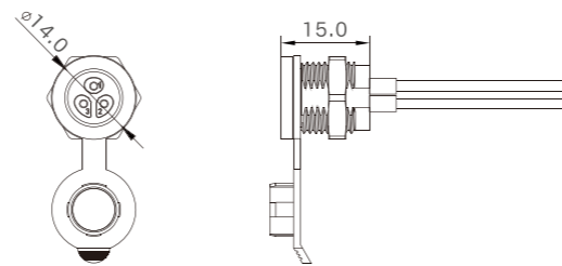
Female Size
