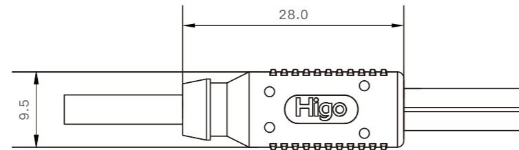
Maximum Diameter
