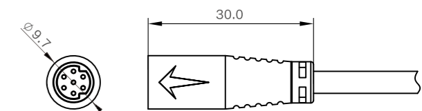
Female Size
