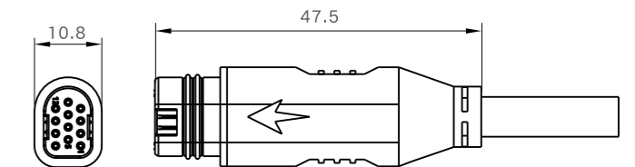
Female Size
