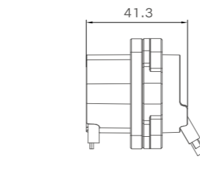
Mating Size
