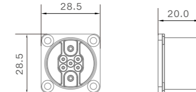
Male Size
