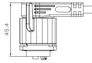
Mating Size
