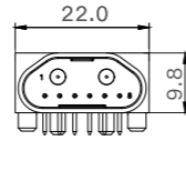
Female Size
