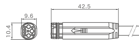
Female Size
