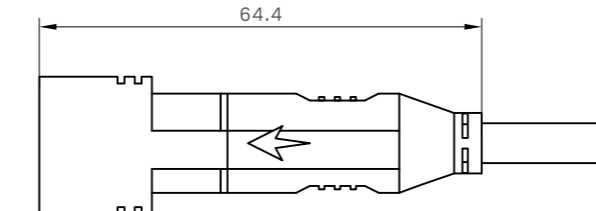
Mating Size
