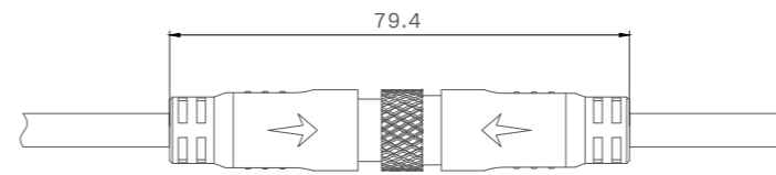
Mating Size
