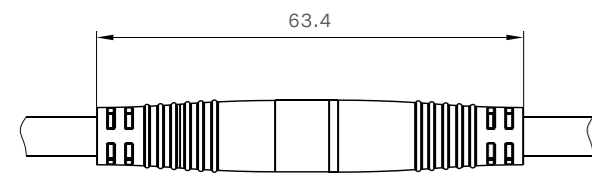
Mating Size
