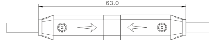
Mating Size
