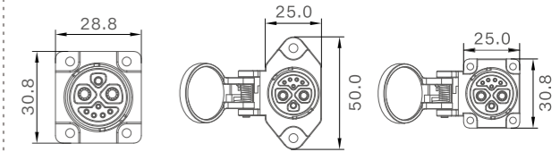
Female Size
