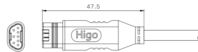
Female Size
