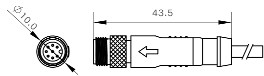
Male Size
