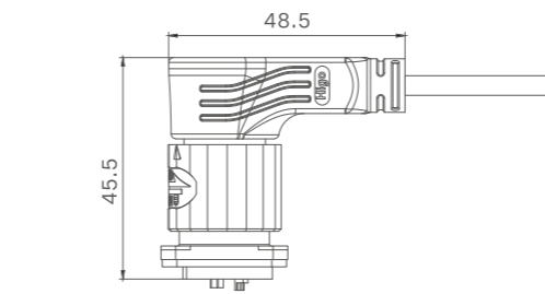
Mating Size
