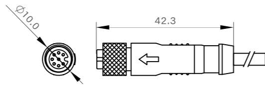
Female Size
