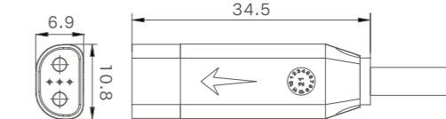
Male Size
