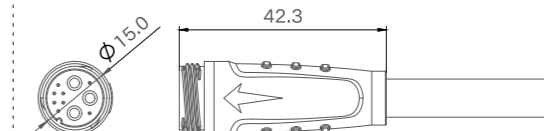
Male Size
