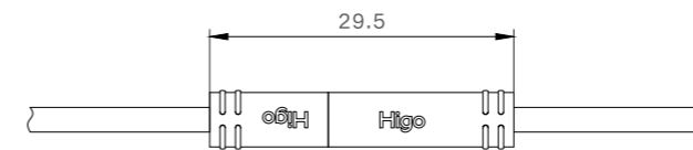
Mating Size
