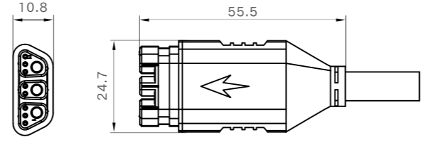
Female Size
