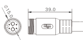
Male Size
