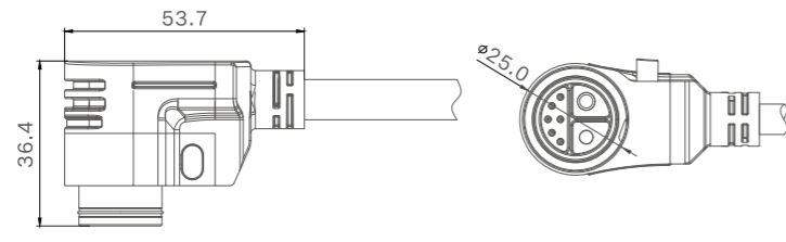
Male Size
