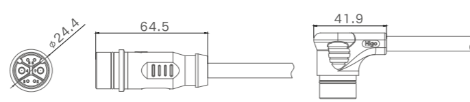
Male Size
