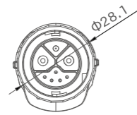
Male Size
