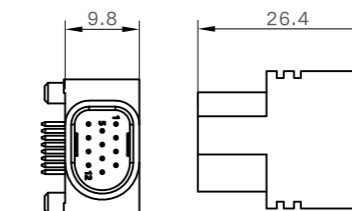
Male Size
