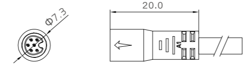
Female Size
