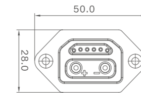
Female Size
