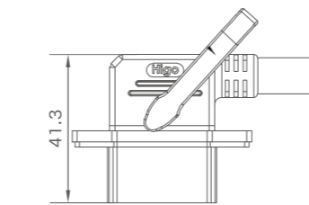
Mating Size
