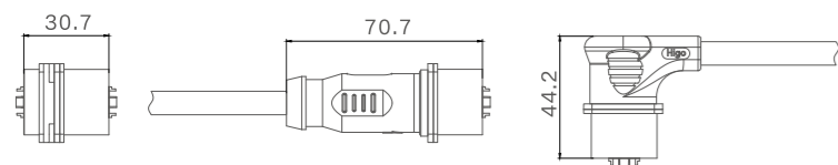
Mating Size
