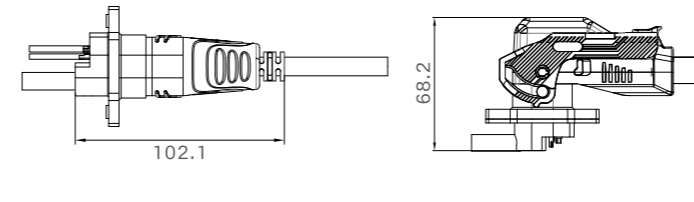
Mating Size
