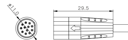
Male Size
