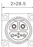
Female Size
