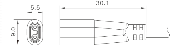
Female Size
