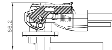
Mating Size
