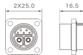
Female Size
