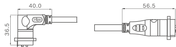
Mating Size
