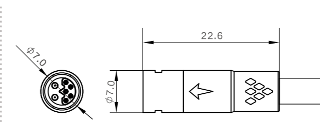
Male Size
