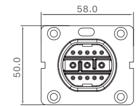
Female Size
