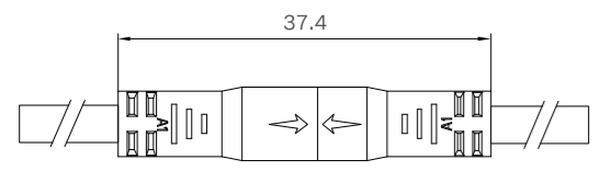
Mating Size
