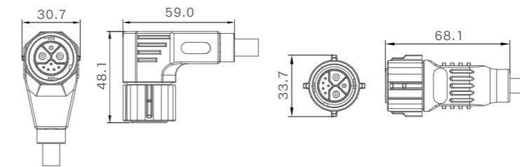
Male Size
