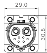
Female Size
