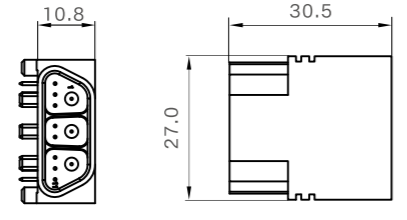
Male Size
