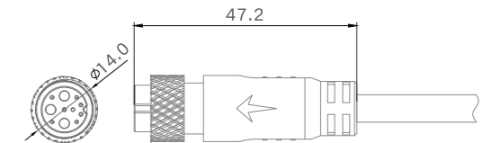
Female Size
