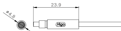
Female Size
