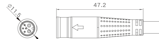
Female Size
